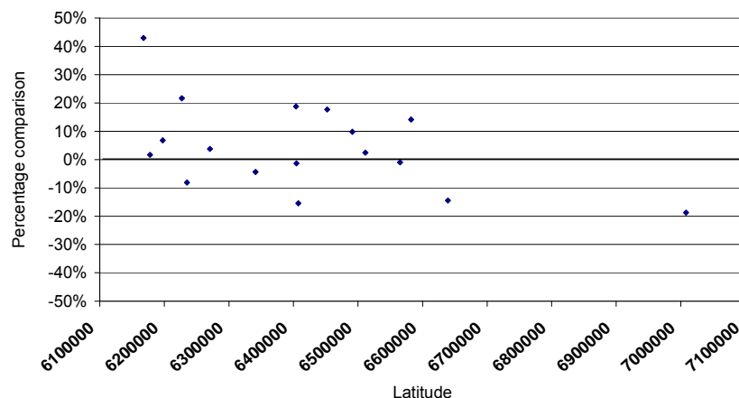
Figure 25 Comparison between the calculated and monitored PM 10 concentrations in percent in the towns shown in Figure 24. The dotted lines are \pm 20\% limitation.
