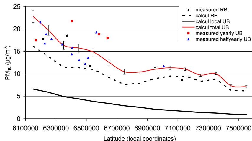
Figure 15 Measured concentrations of total PM 10 in regional background (RB) and urban background (UB) air compared to calculated local, regional and total (local+regional) urban background (UB) concentrations. The error bars show the standard deviation.
